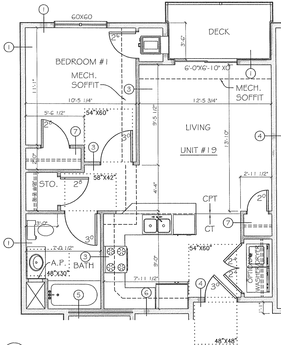
1 TYPICAL PLAN - 1 SCALE: 3/16" = 1'-0"
