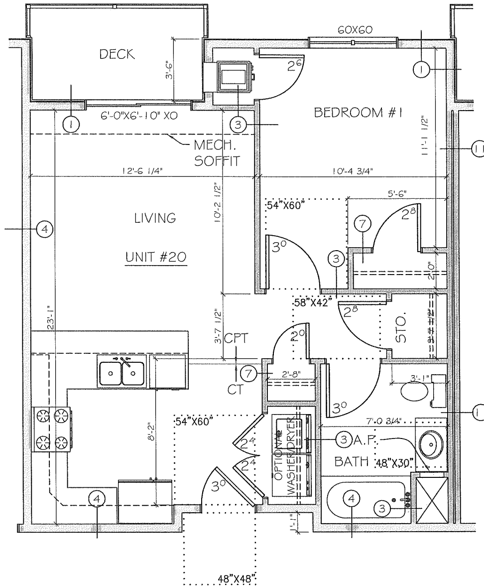
1 TYPICAL PLAN - 2 SCALE: 3/16" = 1'-0"
