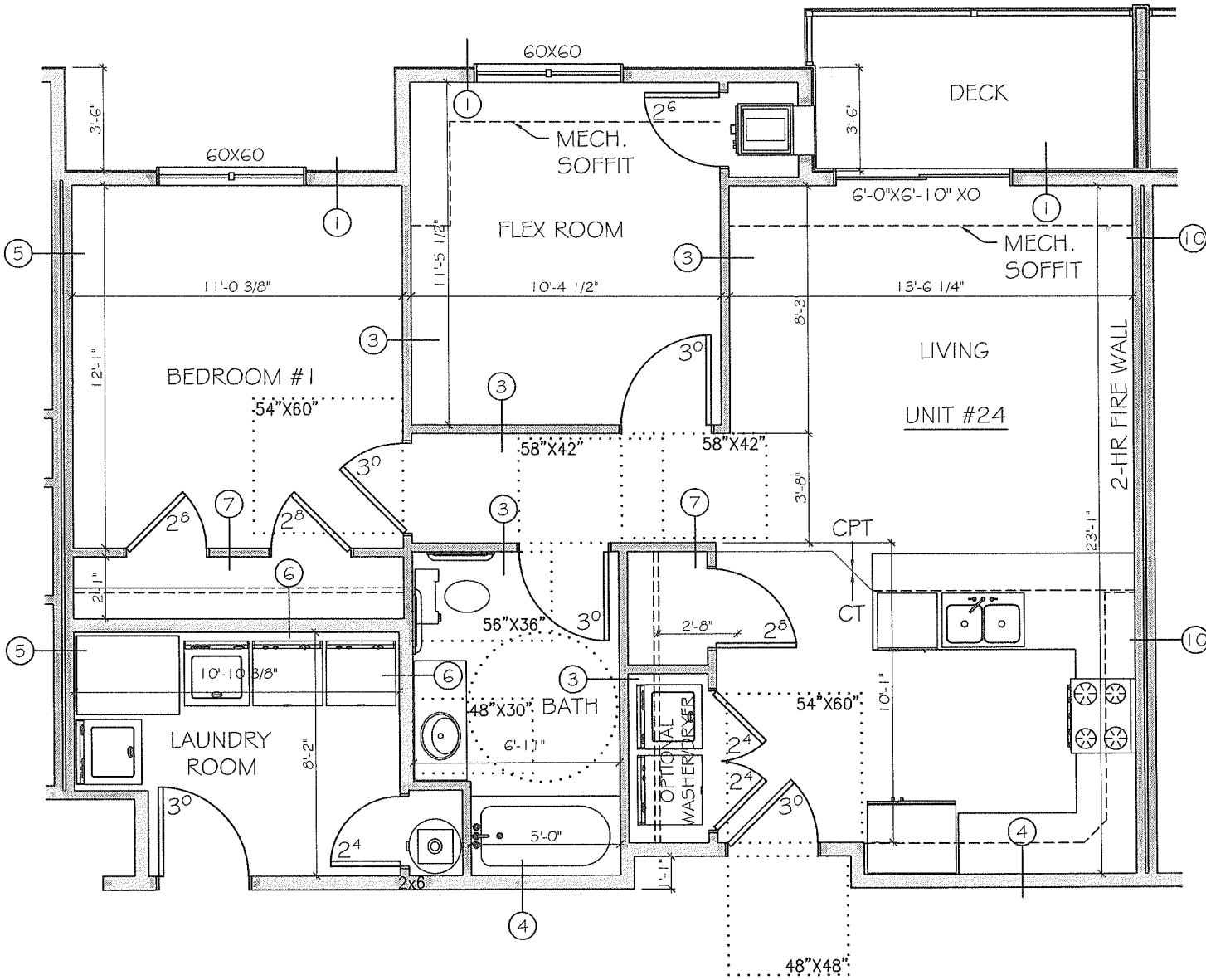
1 TYPICAL PLAN - 4 SCALE: 3/16" = 1'-0"
