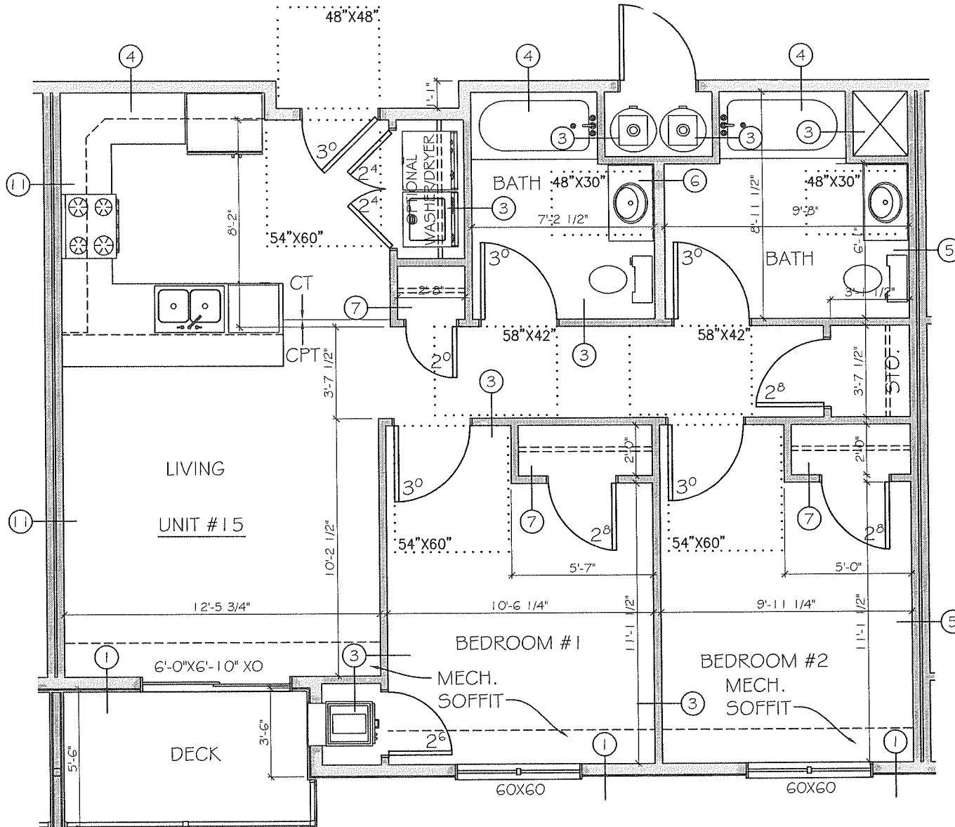
1 TYPICAL PLAN - 6 SCALE: 3/16" = 1'-0"
